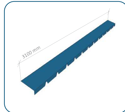
Remate perfurado P5G
